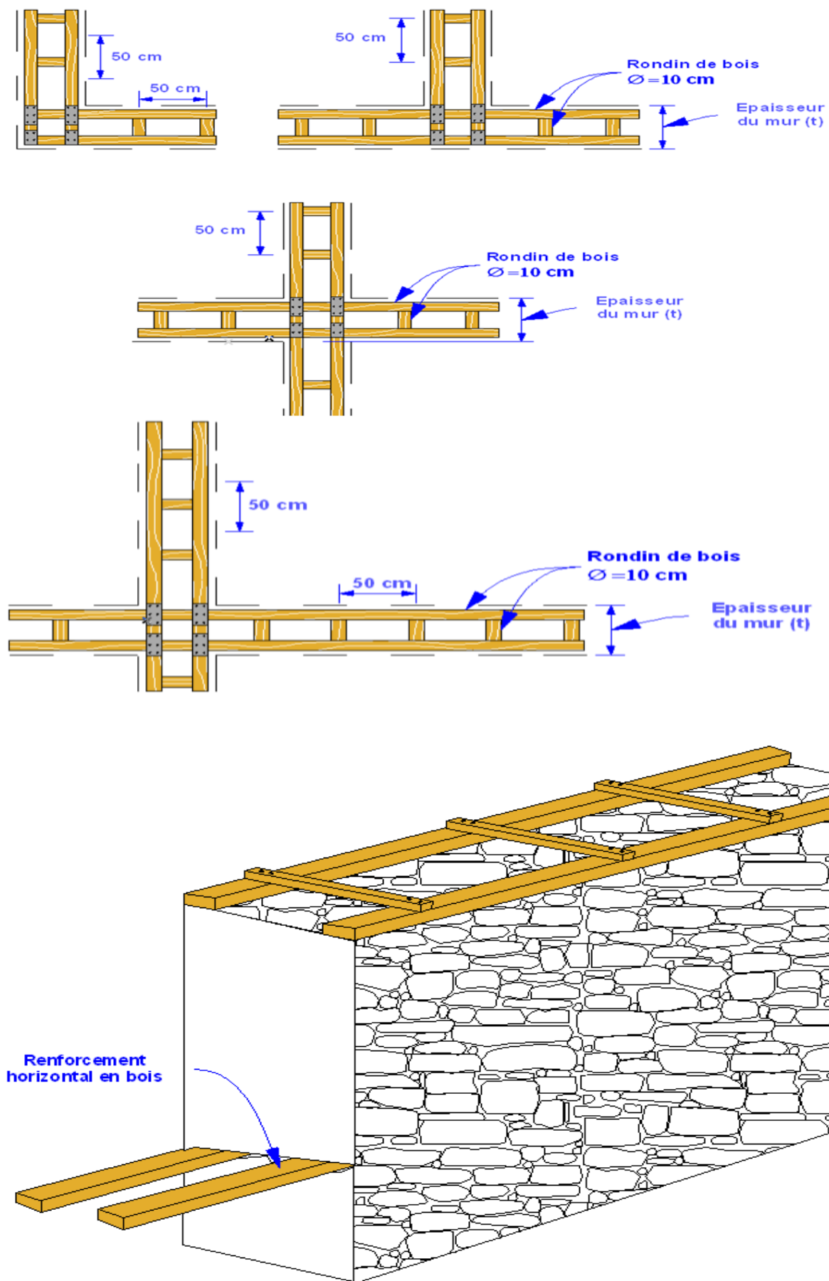
Fig.34. Renforcement horizontal
